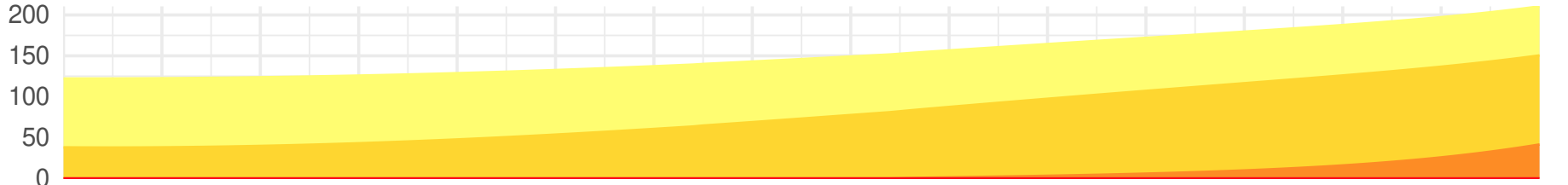
High Emissions (SSP3-7.0)
